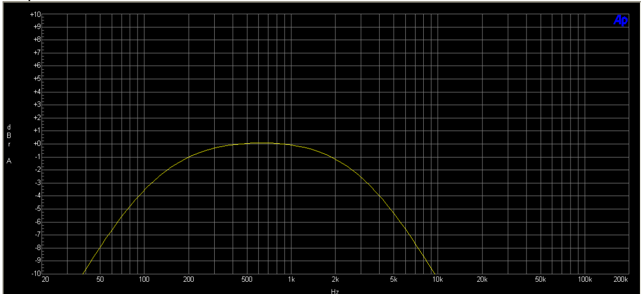
Figure 13: Filter Plot for Compressor Sidechain Filter, Mid-Low Trigger Frequency
